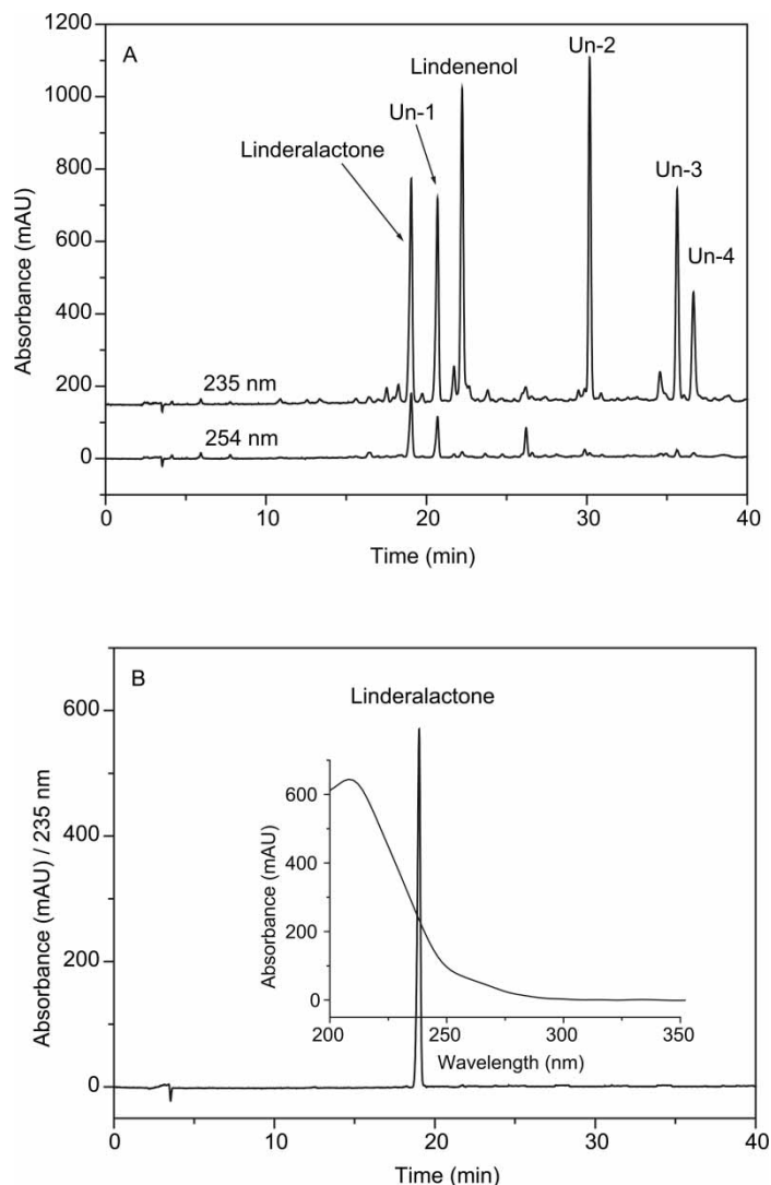
Figure 2. HPLC chromatogram of crude extract from Radix linderae and HSCCC peak fractions. Column: SPHERIGEL ODS C_{18} column (250 mm \times 4.6 mm I.D., 5 \mu m); mobile phase: acetonitrile and water in gradient mode (acetonitrile: water (v/v) from 30:70 to 84:16, in 30 min); flow rate: 1.0 mL \text{min}^{-1} ; detection wavelength: 235 nm and 254 nm; (A) crude extract from Radix linderae ; (B) peak I; (C) peak II of Fig. 3.
