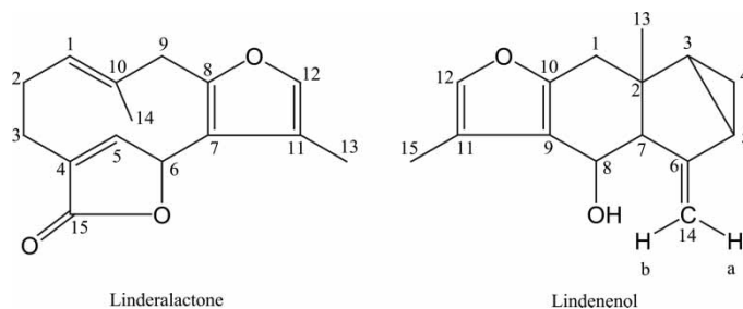
Figure 1. Chemical structures of linderalactone and lindenenol from Radix linderae .
