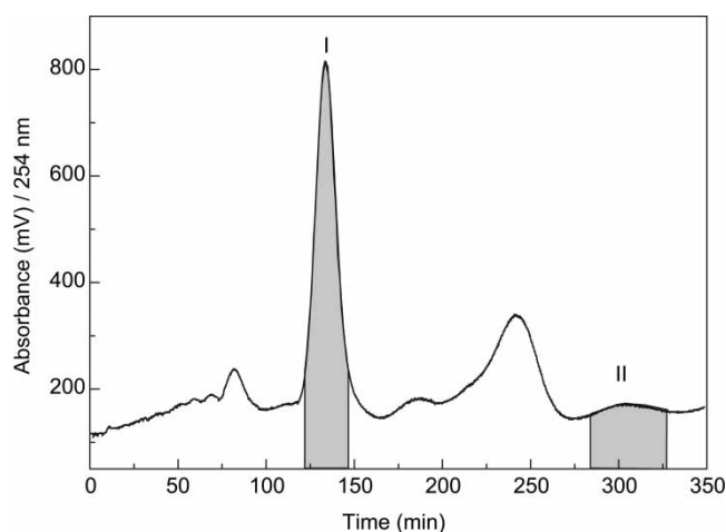
Figure 3. HSCCC chromatogram of crude extract from Radix linderiae . Two phase solvent system: light petroleum-ethyl acetate-methanol-water (5:5:6:4, v/v); mobile phase: the lower phase; flow rate: 2.0 mL min -1 ; revolution speed: 850 rpm; sample size: 450 mg crude extract dissolved in 2 mL of the upper phase and 2 mL of the lower phase of the two phase solvent system; separation temperature: 25°C; retention of the stationary phase: 50%. I: linderalactone (collected during 122–147 min); II: lindenenol (collected during 283–327 min).
